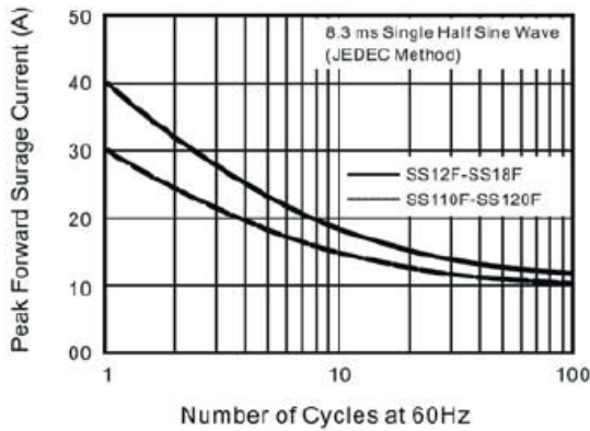
Maximum Non-Repetitive Peak Forward Surge Current
