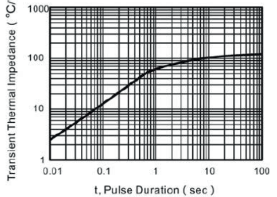
Typical Transient Thermal Impedance
