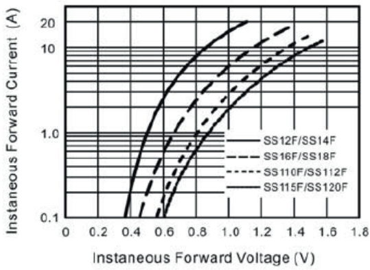
Typical Forward Characteristic
